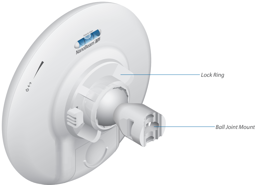
NBE-M5-16 with Mounting Hardware
