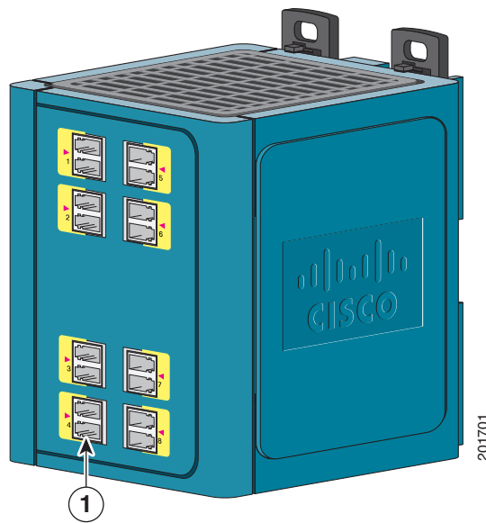
Figure 1-4 Cisco IEM-3000-8FM Expansion Module
