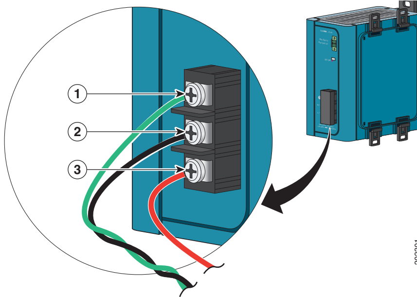
Figure B-44 AC/DC Power Input Terminal Block Wire Connections to a DC Source
