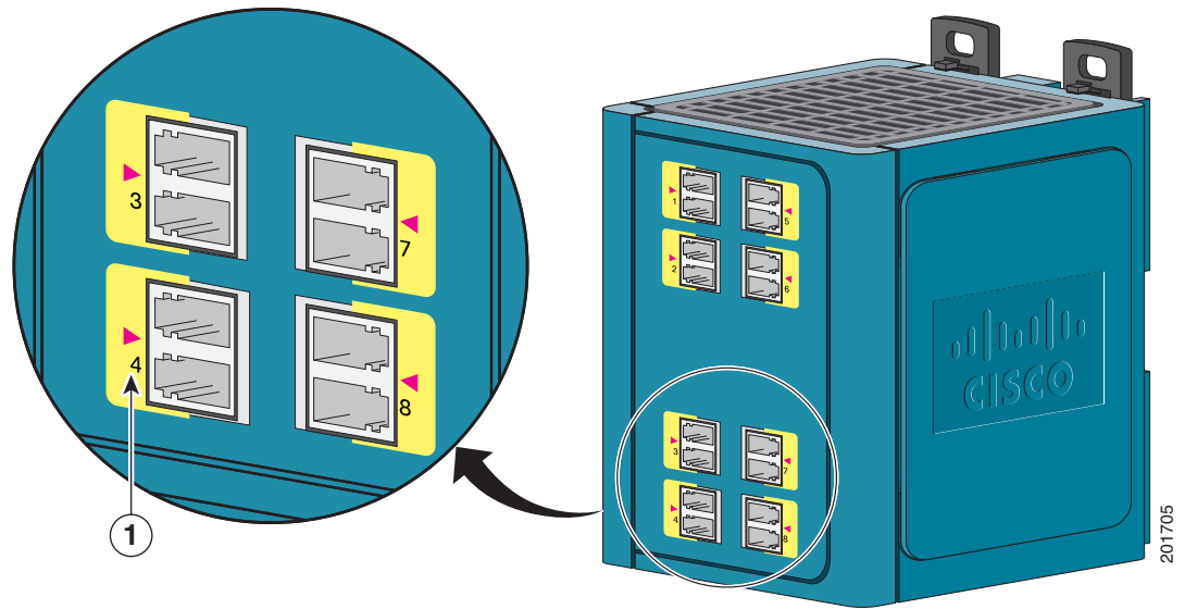
Figure 1-12 LEDs on the Cisco IEM-3000-8FM Module
