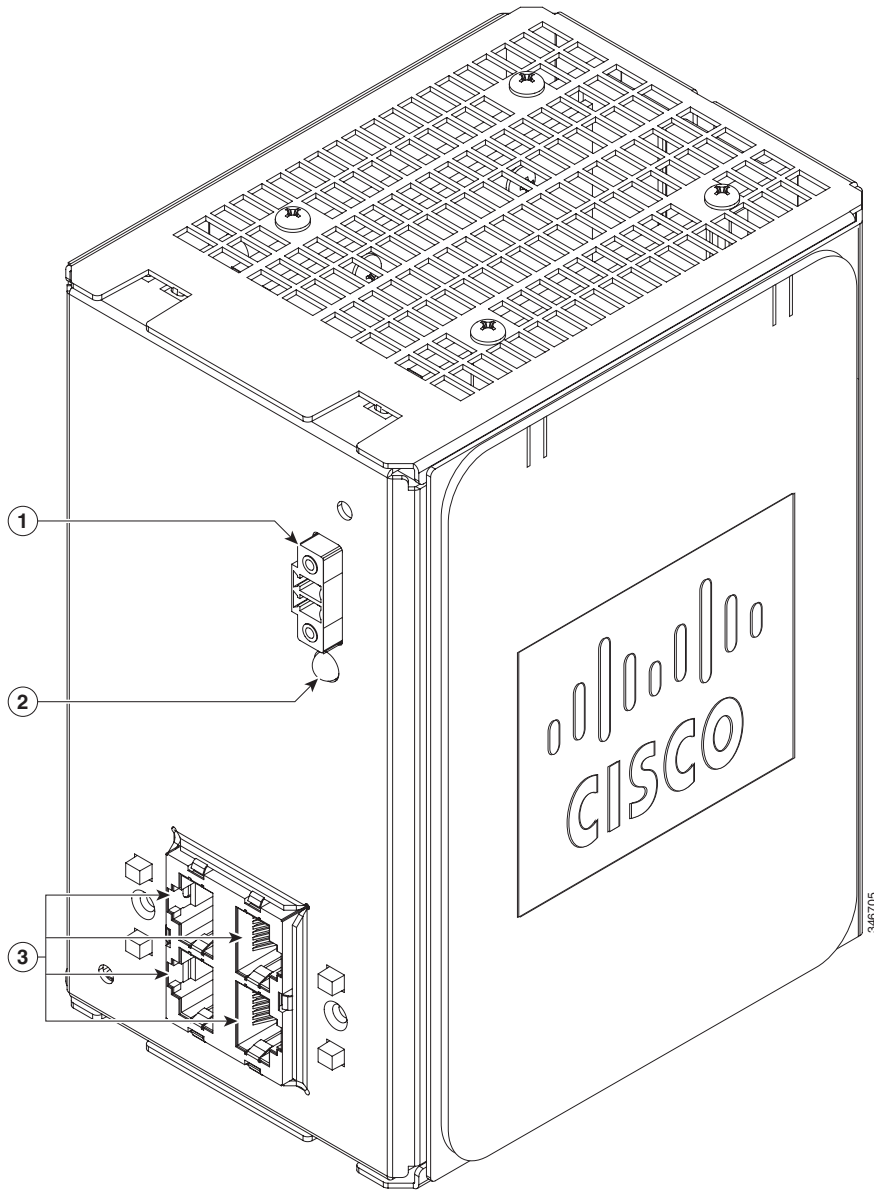
Figure 1-7 Cisco IEM-3000-4PC PoE Expansion Module
