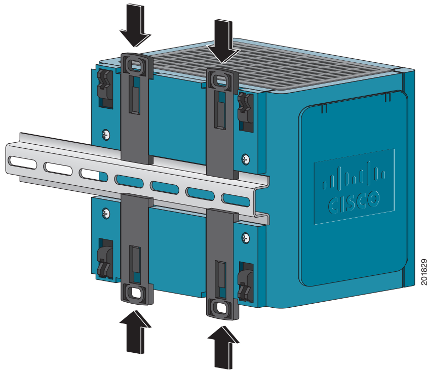
Figure 2-21 Pushing the DIN Rail Latches In
