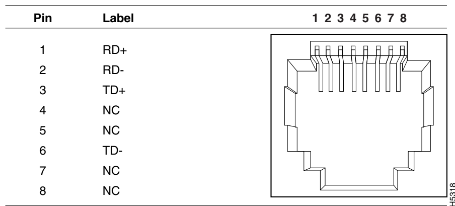
Figure C-1 10/100 Port Pinouts
