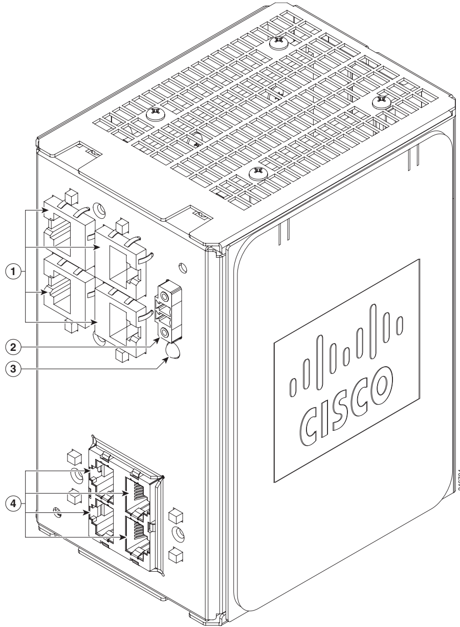
Figure 1-8 Cisco IEM-3000-4PC-4TC PoE Expansion Module
