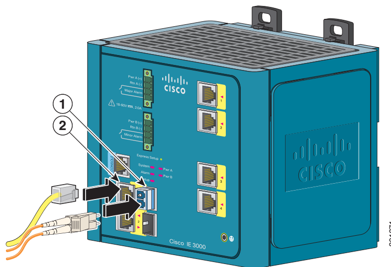
Figure B-36 Connecting to a Dual-Purpose Port
