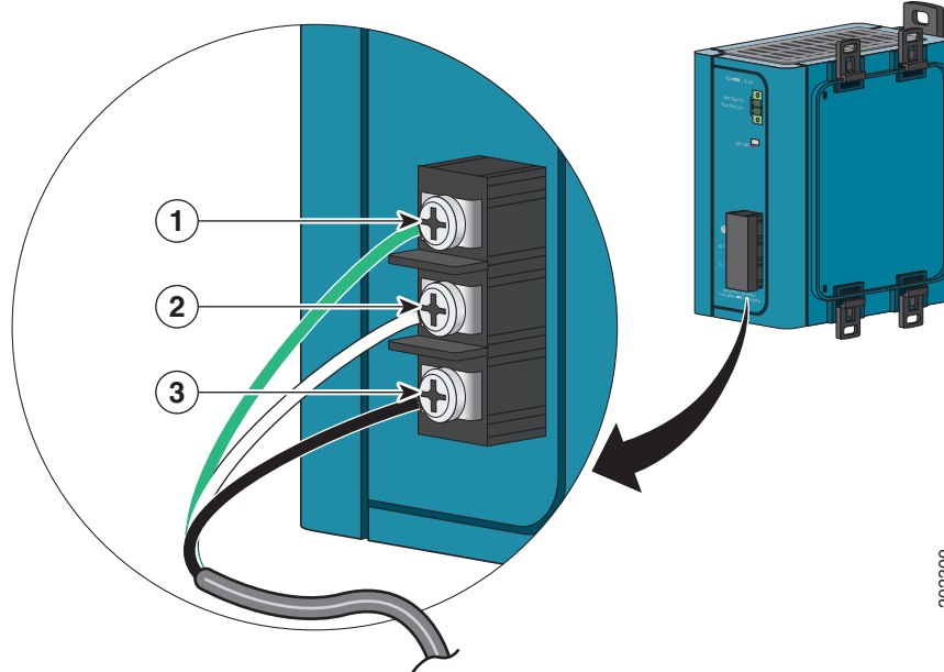
Figure B-43 Connecting AC Power to the Power Converter
