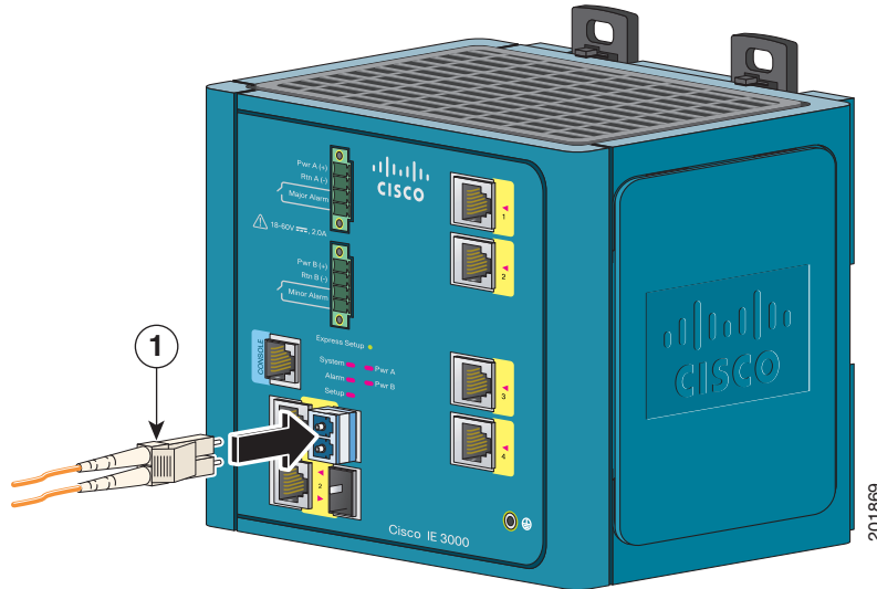
Figure B-35 Connecting to a Fiber-Optic SFP Transceiver Port
