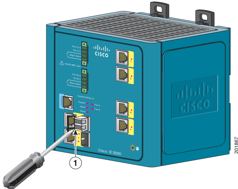
Figure B-34 Removing a Bale-Clasp Latch SFP Transceiver by Using a Flat-Blade Screwdriver
