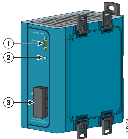
Figure 1-17 Cisco IE 3000 Switch AC/DC Power Converter
