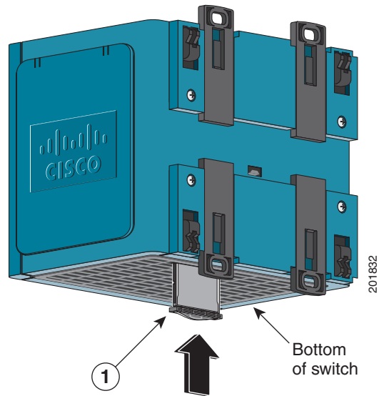
Figure 1-15 Compact Flash Memory Card Slot
