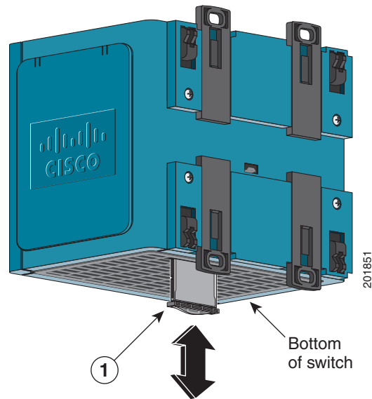
Figure B-7 Removing the Compact Flash Memory Card from the Switch
