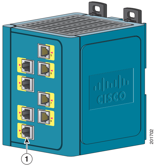
Figure 1-3 Cisco IEM-3000-8TM Expansion Module
