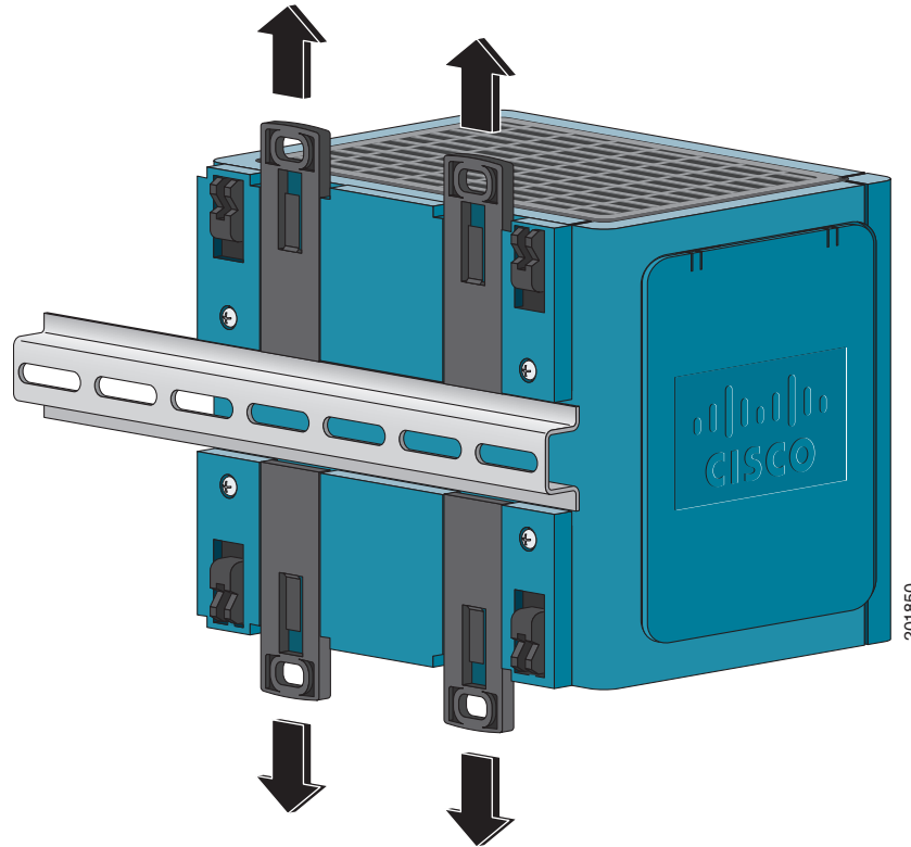
Figure B-27 Removing the Switch from the DIN Rail
