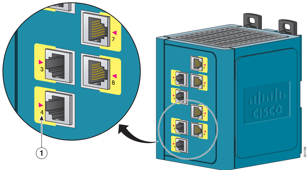
Figure 1-11 LEDs on the Cisco IEM-3000-8TM Module
