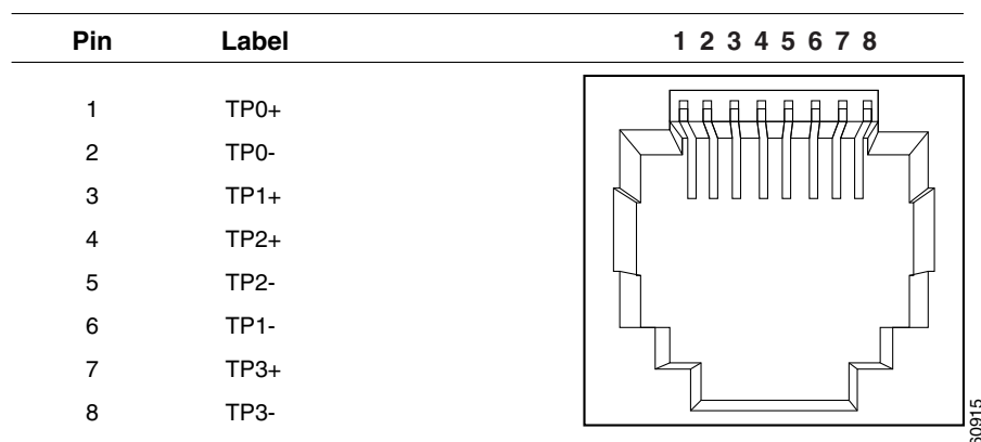
Figure C-2 10/100/1000 Port Pinouts
