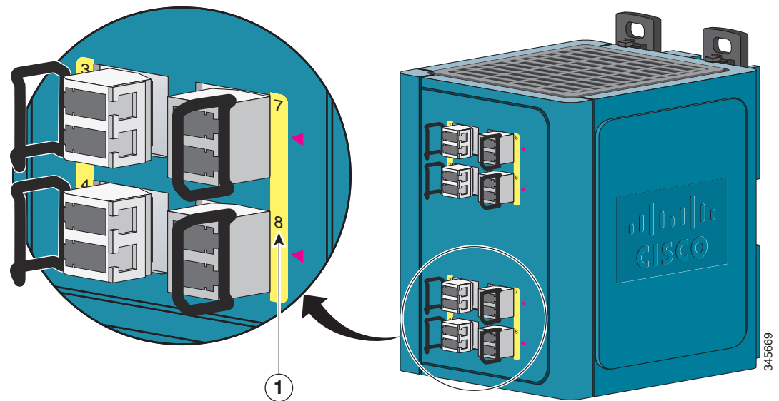
Figure 1-13 LEDs on the Cisco IEM-3000-8SM Module
