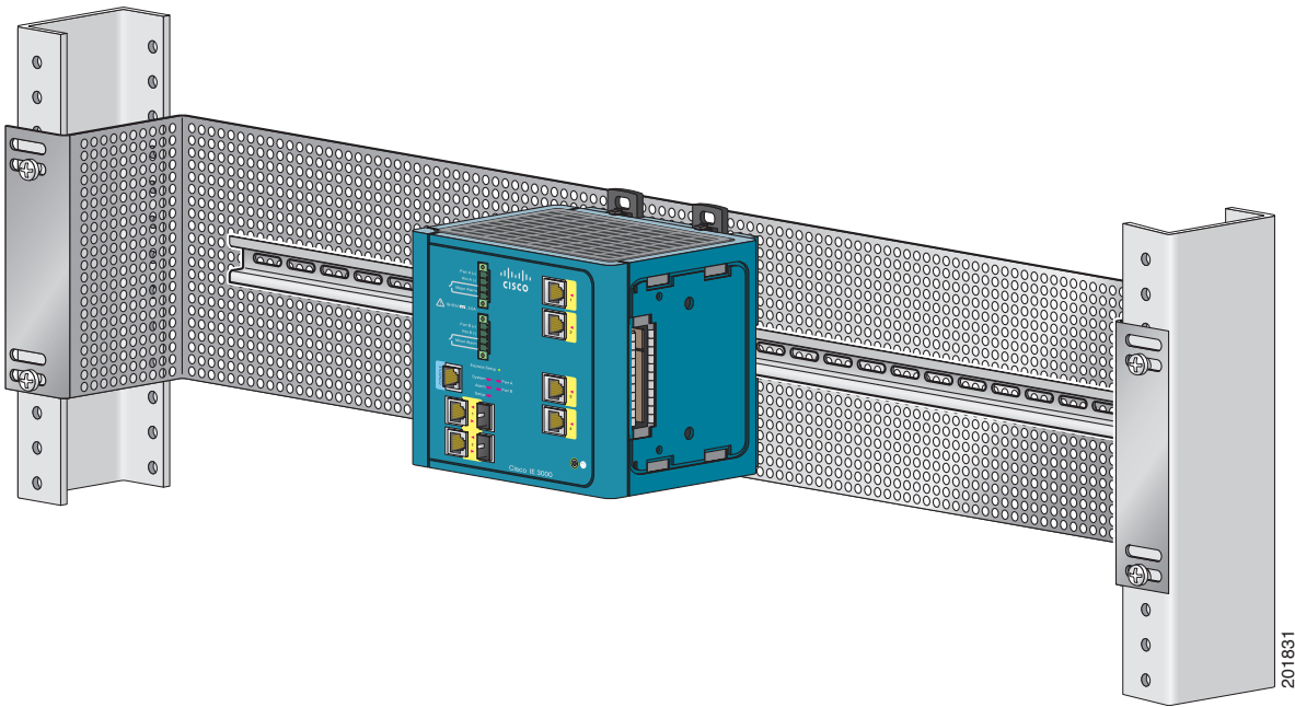
Figure B-26 Installing the Switch on a Rack
