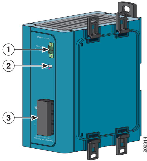
Figure 1-18 AC-Input Power Supply (PWR-IE50W-AC= Shown)
