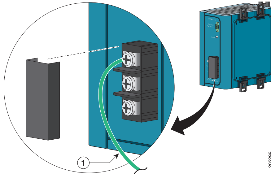
Figure B-42 AC/DC Power Input Terminal Block
