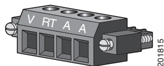
Figure 1-9 Power and Relay Connector
