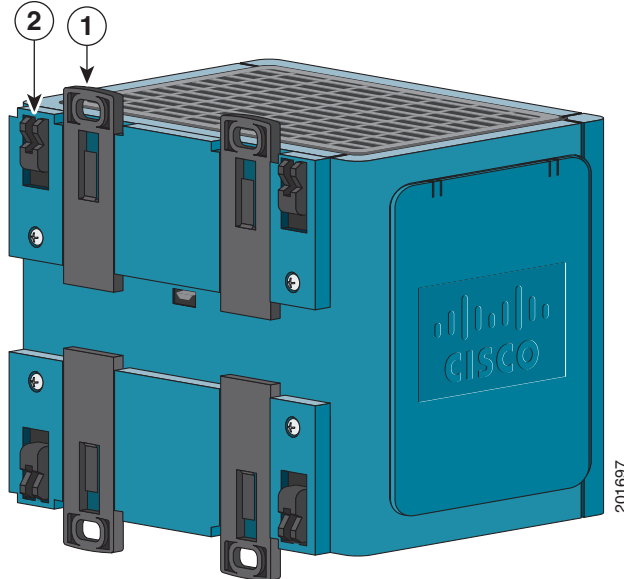
Figure 1-16 Cisco IE 3000 Switch Rear Panel
