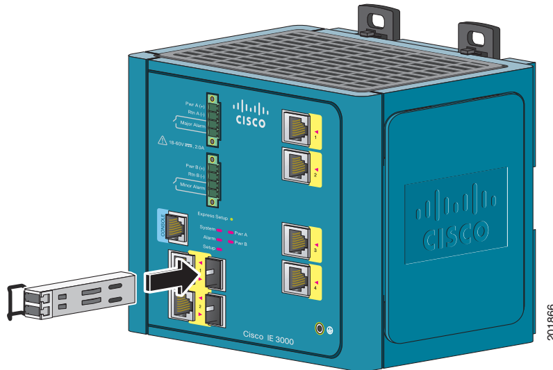
Figure B-33 Installing an SFP Transceiver into an SFP Module Socket
